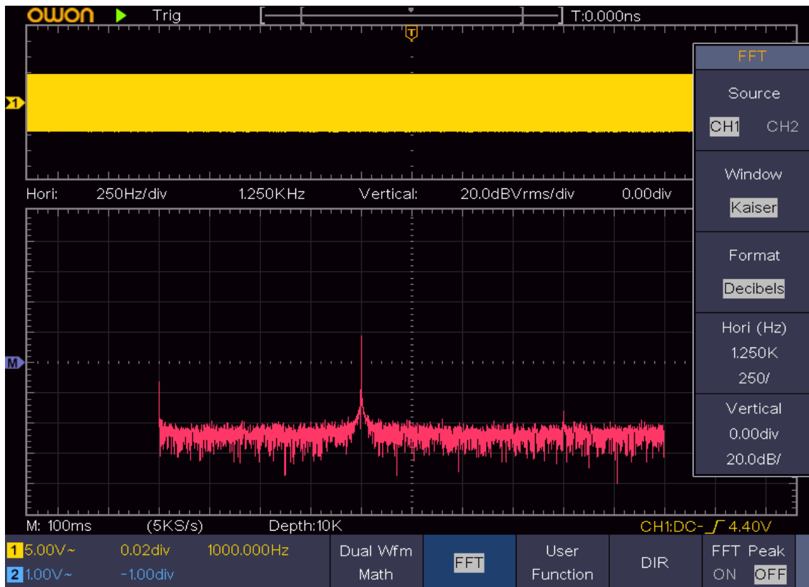
Figure 4-5 Kaiser window
