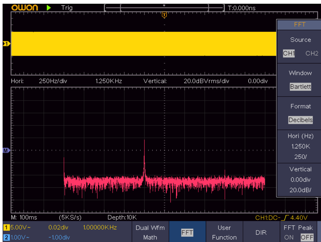
Figure 4-6 Bartlett window
