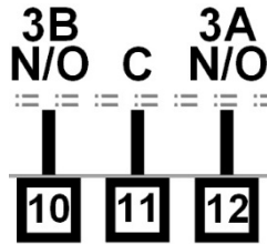
Figure 33. Plug-in Module Slot 3 - Dual Relay Module
