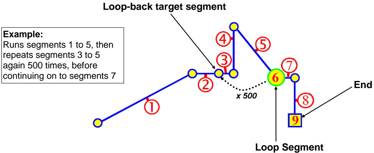
Figure 49. Loop-back Segments
