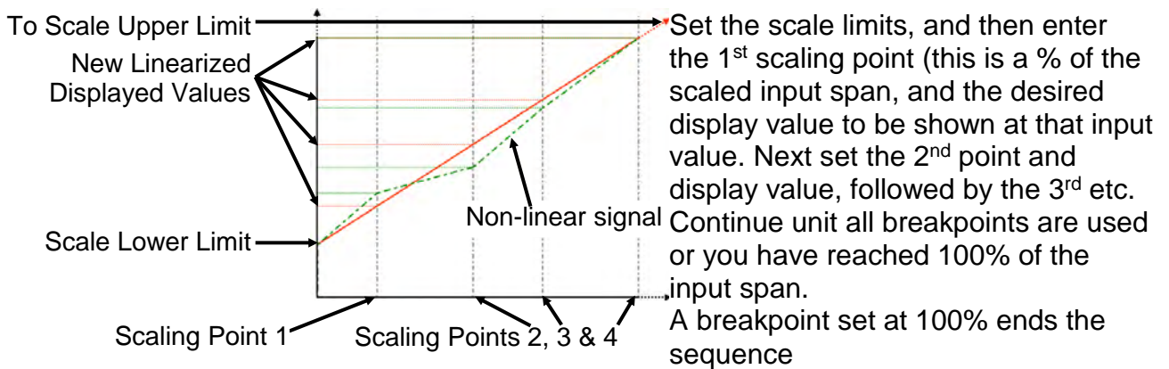
Figure 46. Multi-point Scaling
