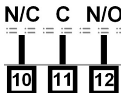
Figure 32. Plug-in Module Slot 3 – Single Relay Module
