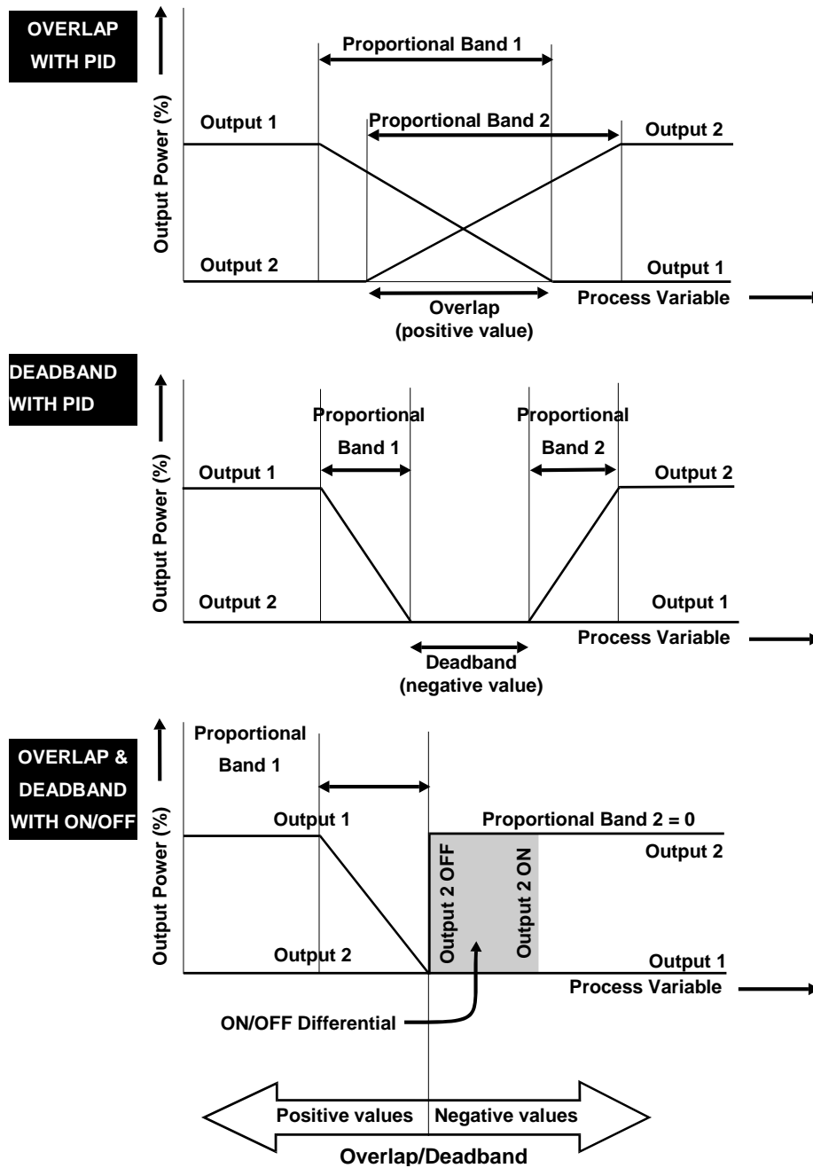
Figure 63. Overlap/Deadband
