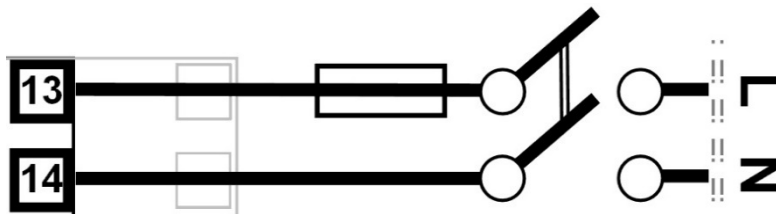
Figure 9. Mains Power Connections
