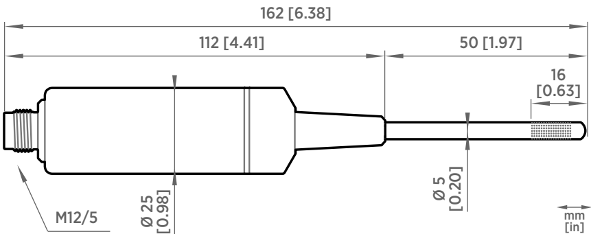
Figure 35 HMP1 probe dimensions
