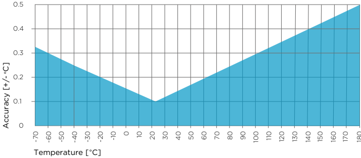
Figure 57 TMP1 temperature measurement accuracy over full range
