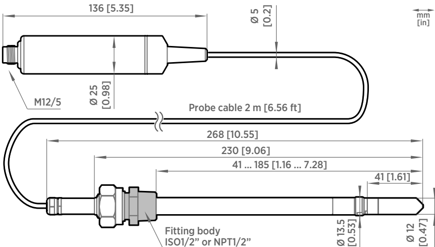
Figure 50 HMP8 probe dimensions
