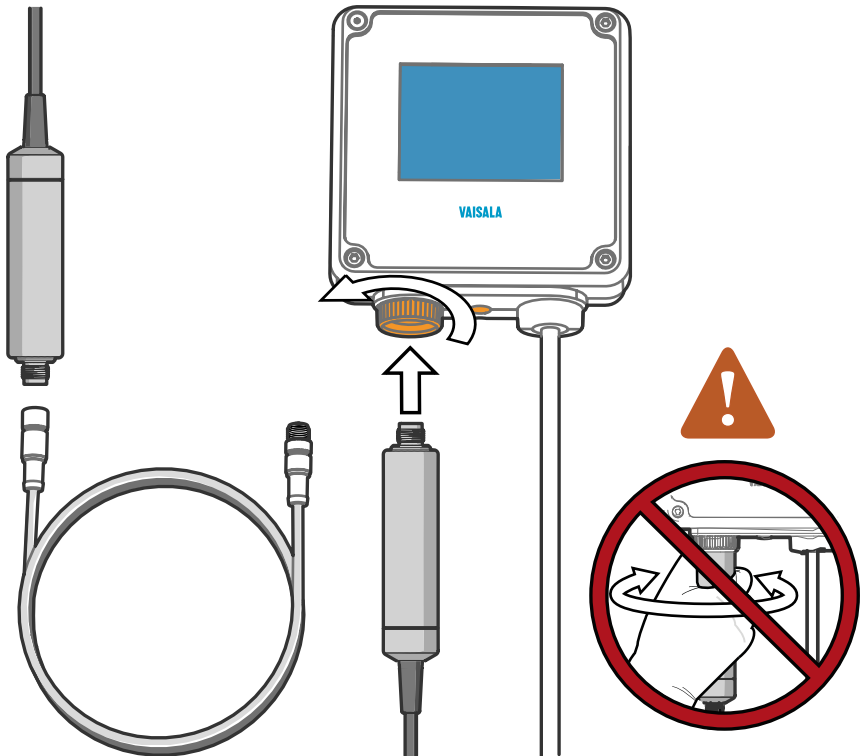
Figure 27 Attaching the probe to Indigo200 series transmitter
