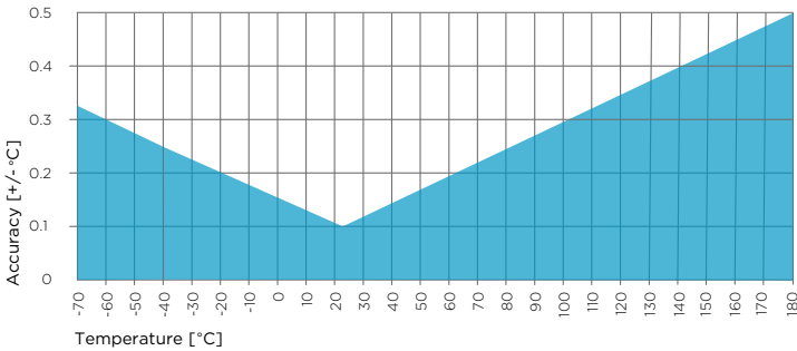
Figure 49 HMP8 temperature measurement accuracy over full range
