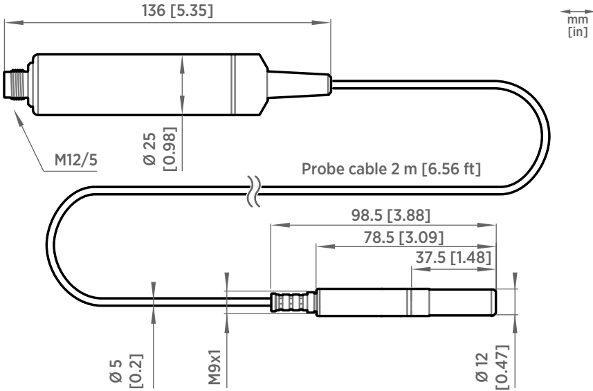
Figure 38 HMP3 probe dimensions
