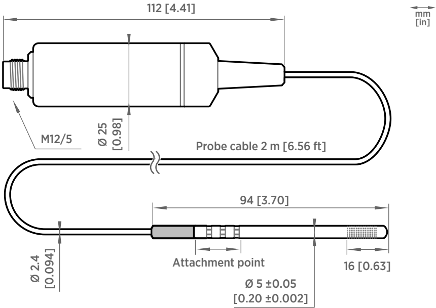
Figure 54 HMP9 probe dimensions
