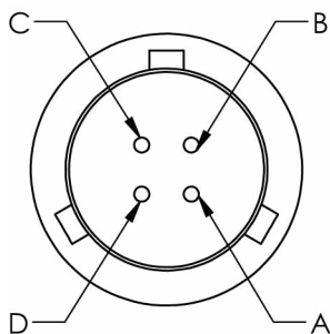
4 PIN BAYONET
