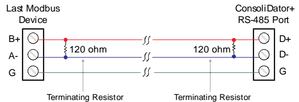
Figure 26. Serial Connections
