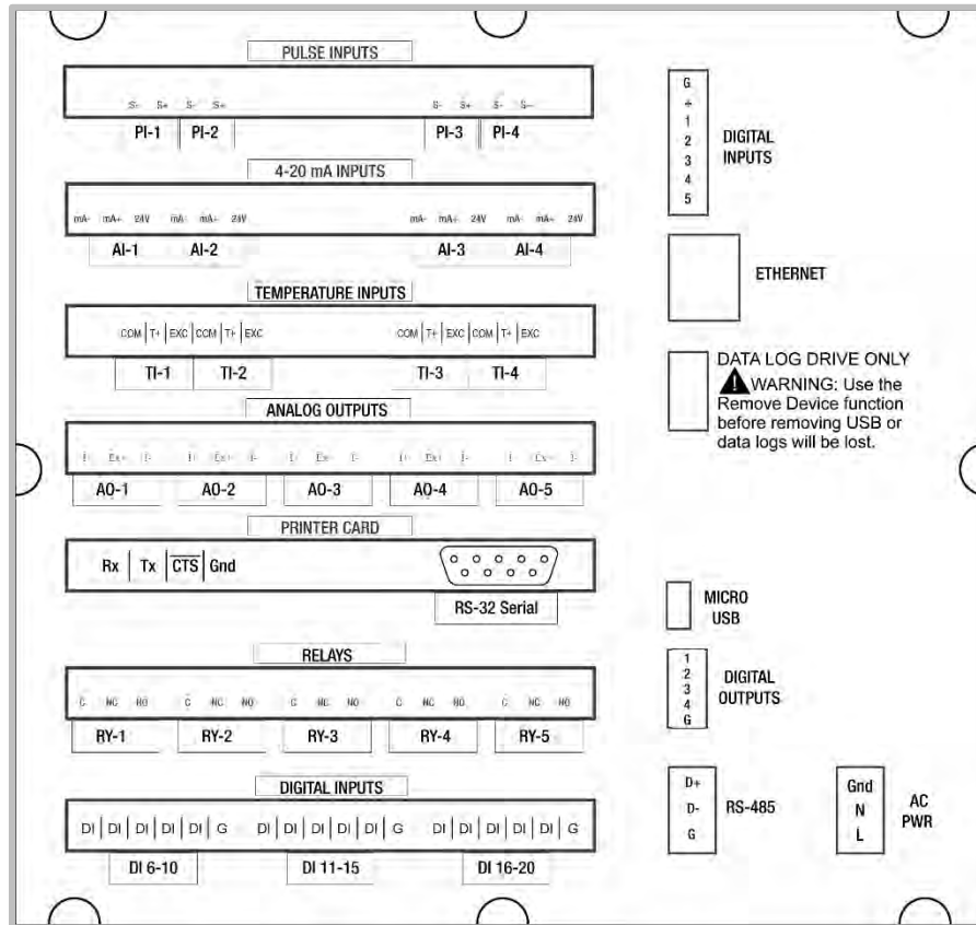
Figure 5. Connection Terminals for a PD9000-6N-4PI-4AI-4TI-5AO-5RY-15DI-E-P
