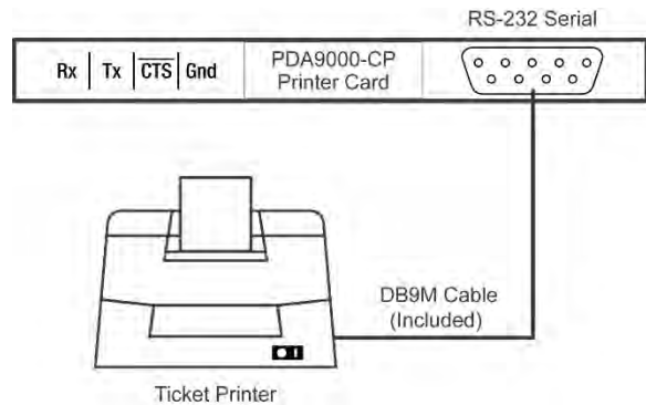
Figure 22. Printer Connections
