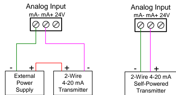
Figure 9. Transmitter Powered by External Supply or Self-Powered
