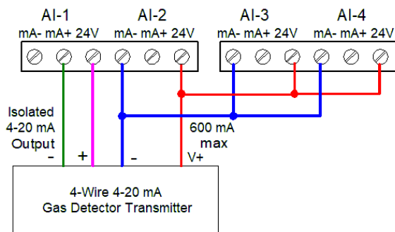
Figure 21. Powering 4-Wire Gas Detector & Isolated 4-20 mA Output
