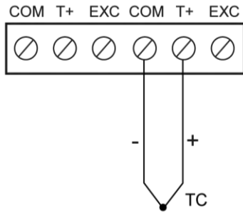
Figure 11. Thermocouple Input Connections
