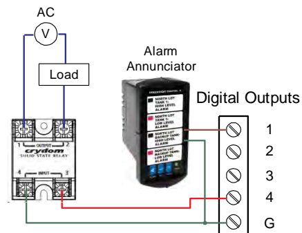
Figure 19. Digital Outputs Driving 5 V Solid State Relay
