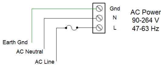
Figure 6. AC Power Connections
