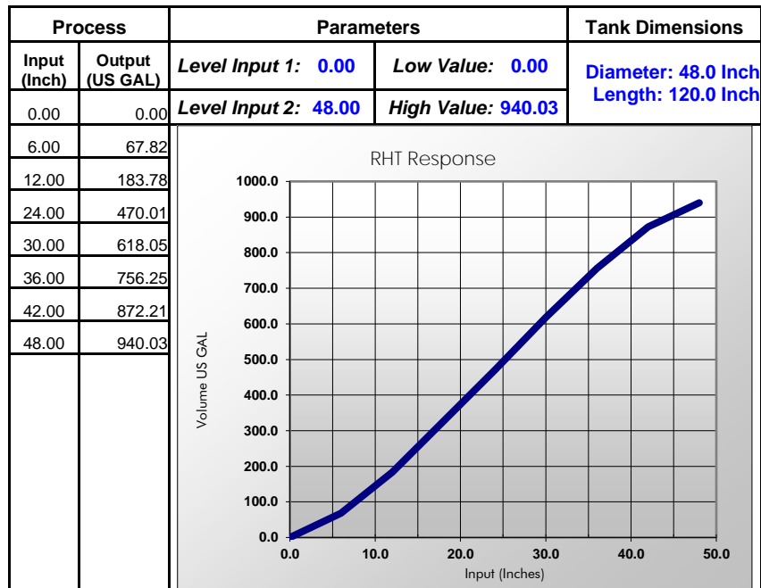
Figure 31. Round Horizontal Tank Volume Graph
