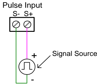
Figure 15. Flow Meter Pulse Input Connections
