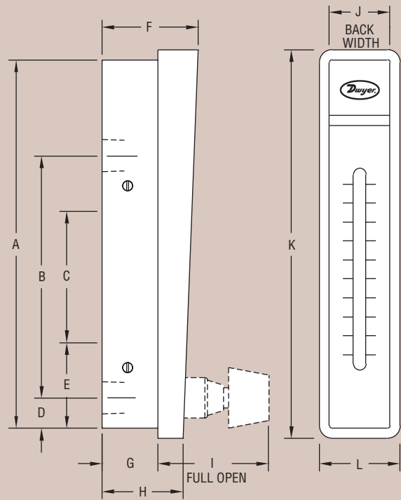
Flowmeter Dimensions
