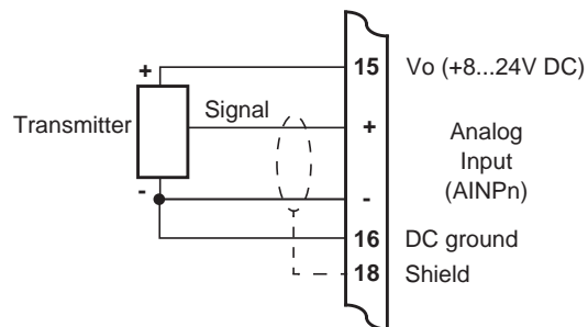
Figure 5 Internally Powered Voltage Transmitter
