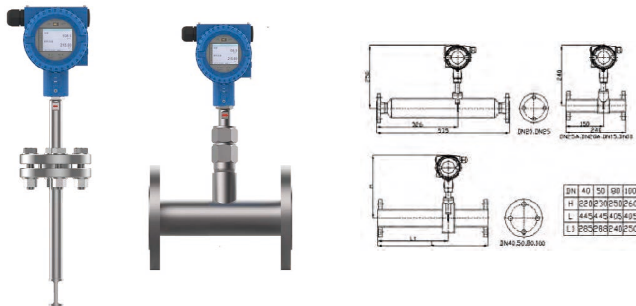
Flanged insertion type
